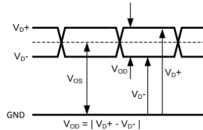
CML Output Signal Levels
